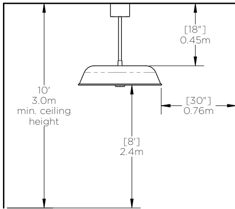
3000W CLEARANCES
