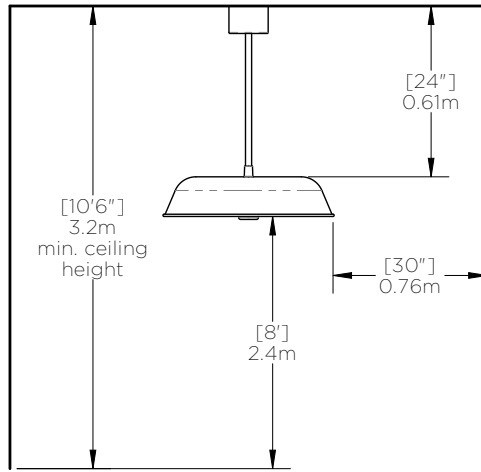
4500W CLEARANCES
